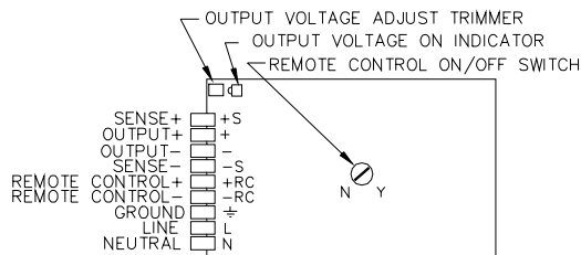
FIGURE 2. COMPONENT LOCATIONS
