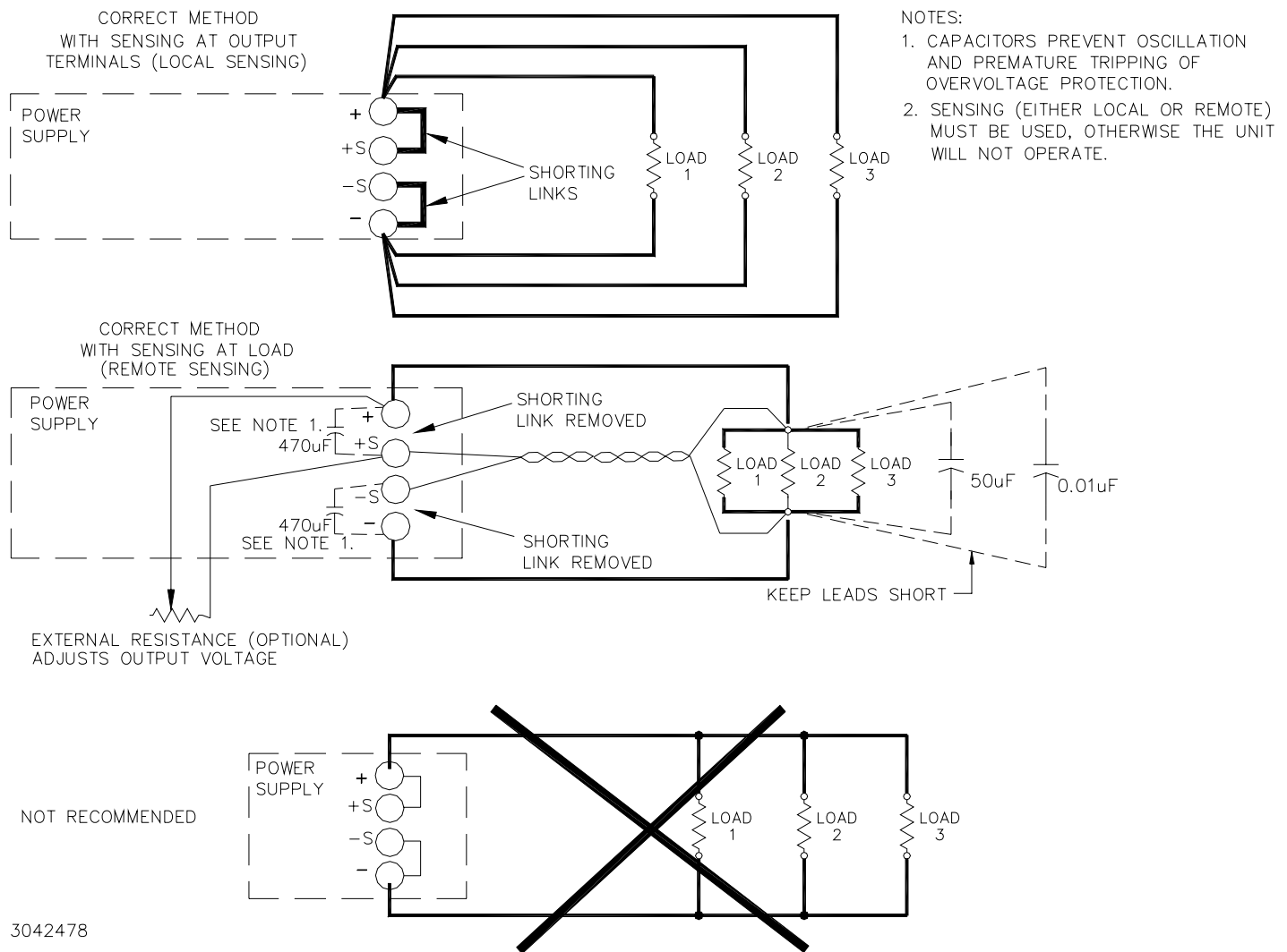
FIGURE 3. LOAD CONNECTIONS
