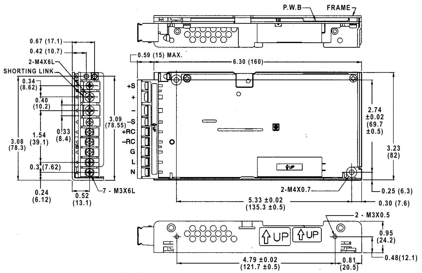
FIGURE 4. POWER SUPPLY MOUNTING
