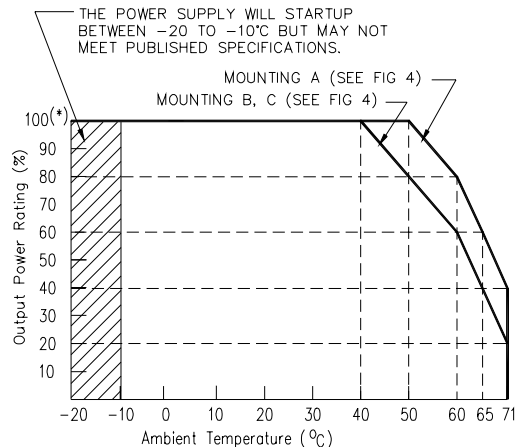
FIGURE 1. OUTPUT POWER VS. TEMPERATURE
